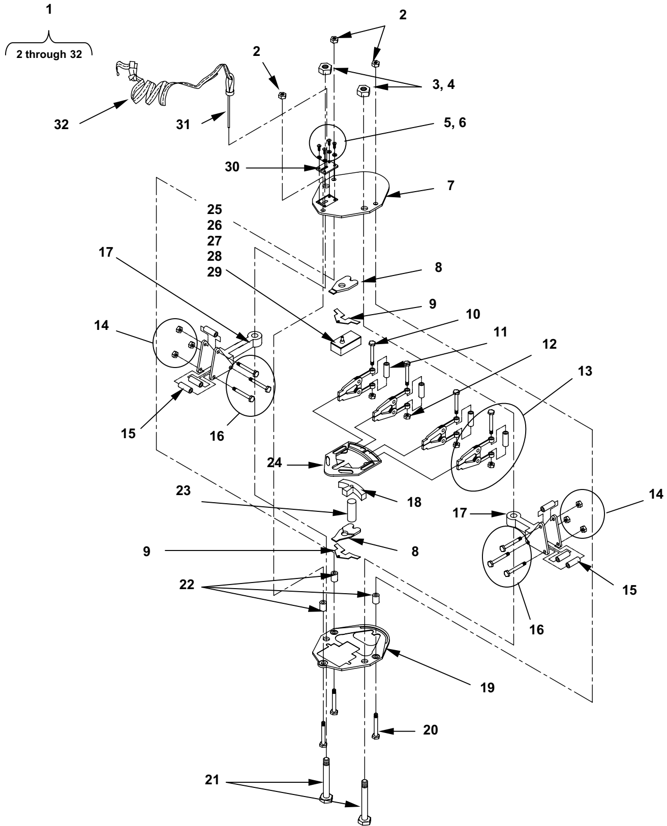
Figure 9. M-1 Cargo Parachute Release
